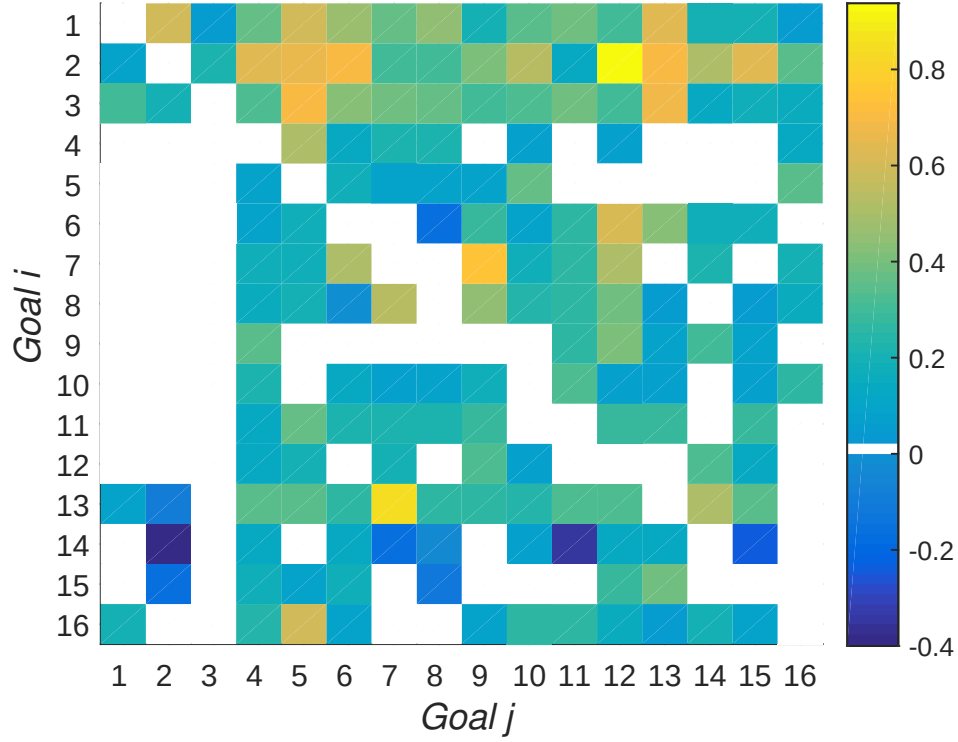
Figure 1: Heat map showing the quantitative values A_{ij} of links between the SDGs, constructed from a detailed analysis of the ICSU report. The colour of the matrix entry with coordinates (i, j) indicates the support that progress on Goal j leads to progress on Goal i . Entries left white indicate an absence of a link. For example, the dark (blue) squares indicating A_{14,2} and A_{14,11} show the significant negative impacts that progress on Goals 2 and 11 is indicated to have on Goal 14, corresponding to the red edges with negative weights in figure 2.
