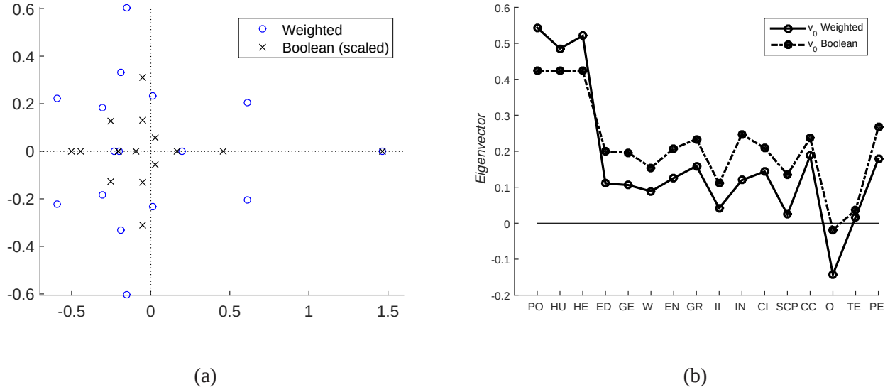
Figure 5: Comparisons between the weighted network and the unweighted (Boolean) version. (a) Eigenvalues of the adjacency matrices A in the complex plane. The eigenvalues of the Boolean case are scaled so that the largest eigenvalues agree, in order to enable a direct comparison. (b). Components of the eigenvectors \mathbf{v}^{(0)} in the two cases, normalised so that \sum_{j=1}^{16} (v_j^{(0)})^2 = 1 .
