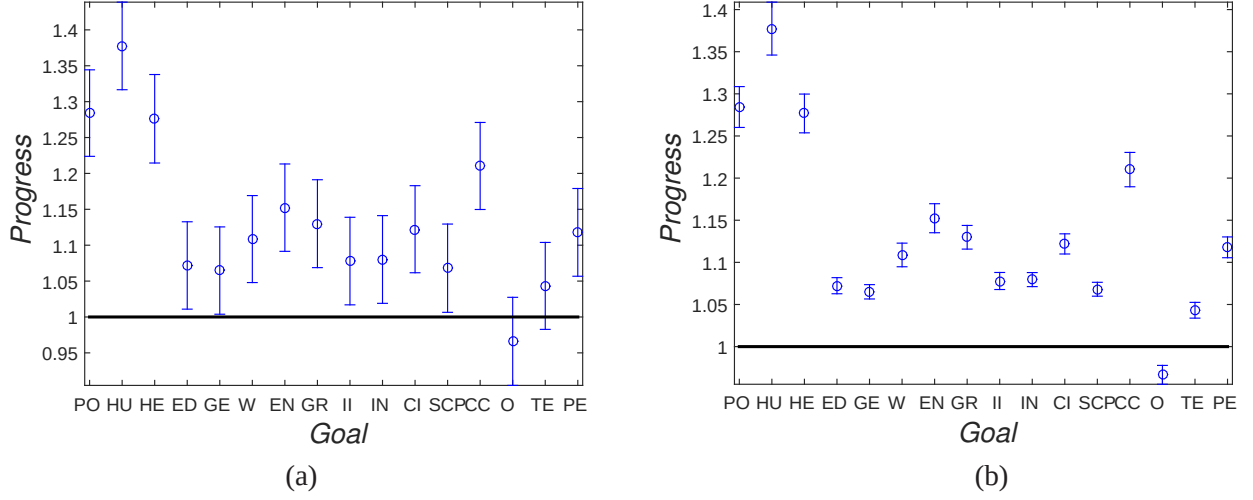
Figure 6: Progress on each SDG when direct efforts are set to m_i = 1 for each i , and the network coupling parameter \varepsilon = 0.1 , indicating indirect effects that are 10% of the strength of direct effects, normalised relative to the uncoupled case \varepsilon = 0 . Circles (in both cases) show expected progress on each Goal, integrating the ODE model (1) from the initial state \mathbf{x}(0) = 1 at t = 0 up to time t = 15 . Error bars illustrate (a) the variation in results due to stochastic perturbations to all the network links in A ; and (b) the variation in results due to stochastic perturbations only to the weightings for the non-zero edges identified in the ICSU Report.
