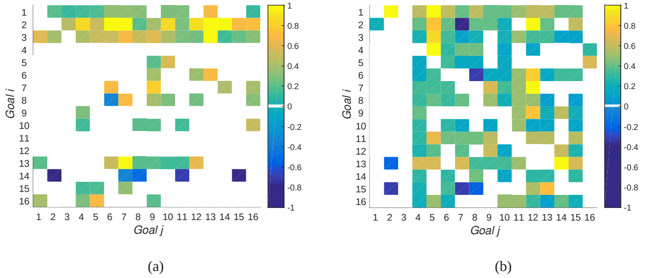
Figure 4: Heat maps showing the quantitative values of links between the SDGs, constructed from the ICSU report. As in figure 1, the colour of the matrix entry with coordinates (i, j) indicates the support that progress on Goal j lends to progress on Goal i . Entries left white indicate an absence of a link. (a) Heat map built up by rows, A_{ij}^{in} showing in row i the influences of other Goals on Goal i ; (b) Heat map built up by columns, A_{ij}^{out} showing in column j the influences of Goal j on the other Goals.
