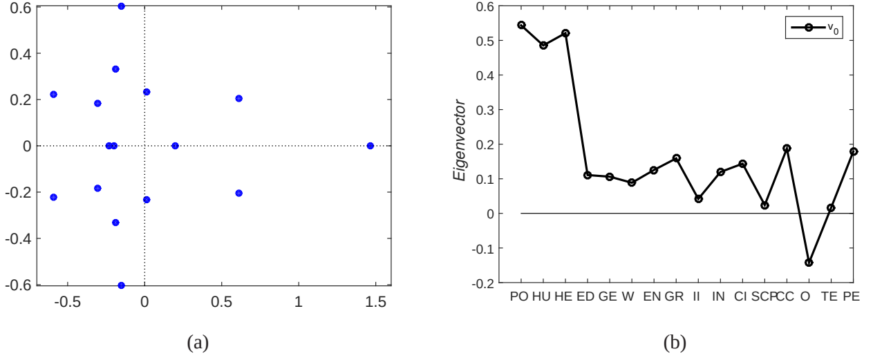
Figure 3: (a) Eigenvalues of A in the complex plane. (b) Components of the eigenvector v^{(0)} corresponding to the leading eigenvalue of A . The eigenvector is normalised so that \sum_{j=1}^{16} \left(v_j^{(0)}\right)^2 = 1 .
