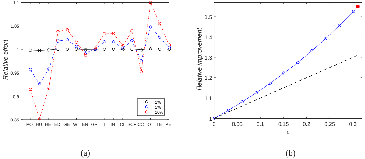
Figure 7: (a). Relative direct effort required on each Goal in order to produce equal total progress by 2030. Results are shown for three different values of \varepsilon : \varepsilon = 0.01 (solid black line), \varepsilon = 0.05 (dashed blue line), and \varepsilon = 0.1 (dash-dotted red line). (b) The optimised level of progress, achieved on every Goal, as the network coupling \varepsilon increases (blue, lower curve). The red square at \varepsilon = 0.311 is the maximum possible value for \varepsilon , see text. The dashed black lines is the straight line 1 + \varepsilon for comparison.
